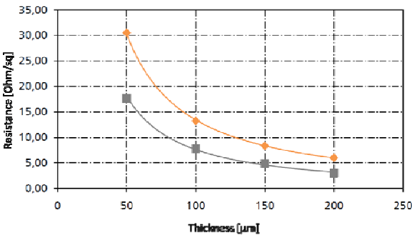
Fig. 8. Carbo e-therm resistance [Ohm/sq] vs. thickness [ \mu\text{m} ].
